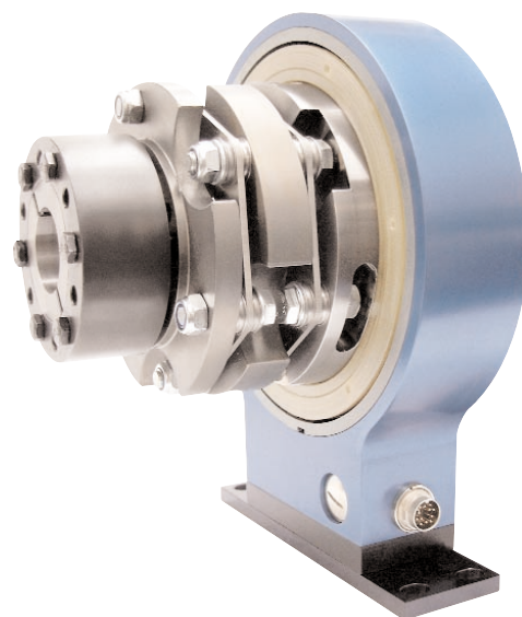
T1 Torque Coupling Rotary Torque Transducer Shown with standard shrink-disk hub
